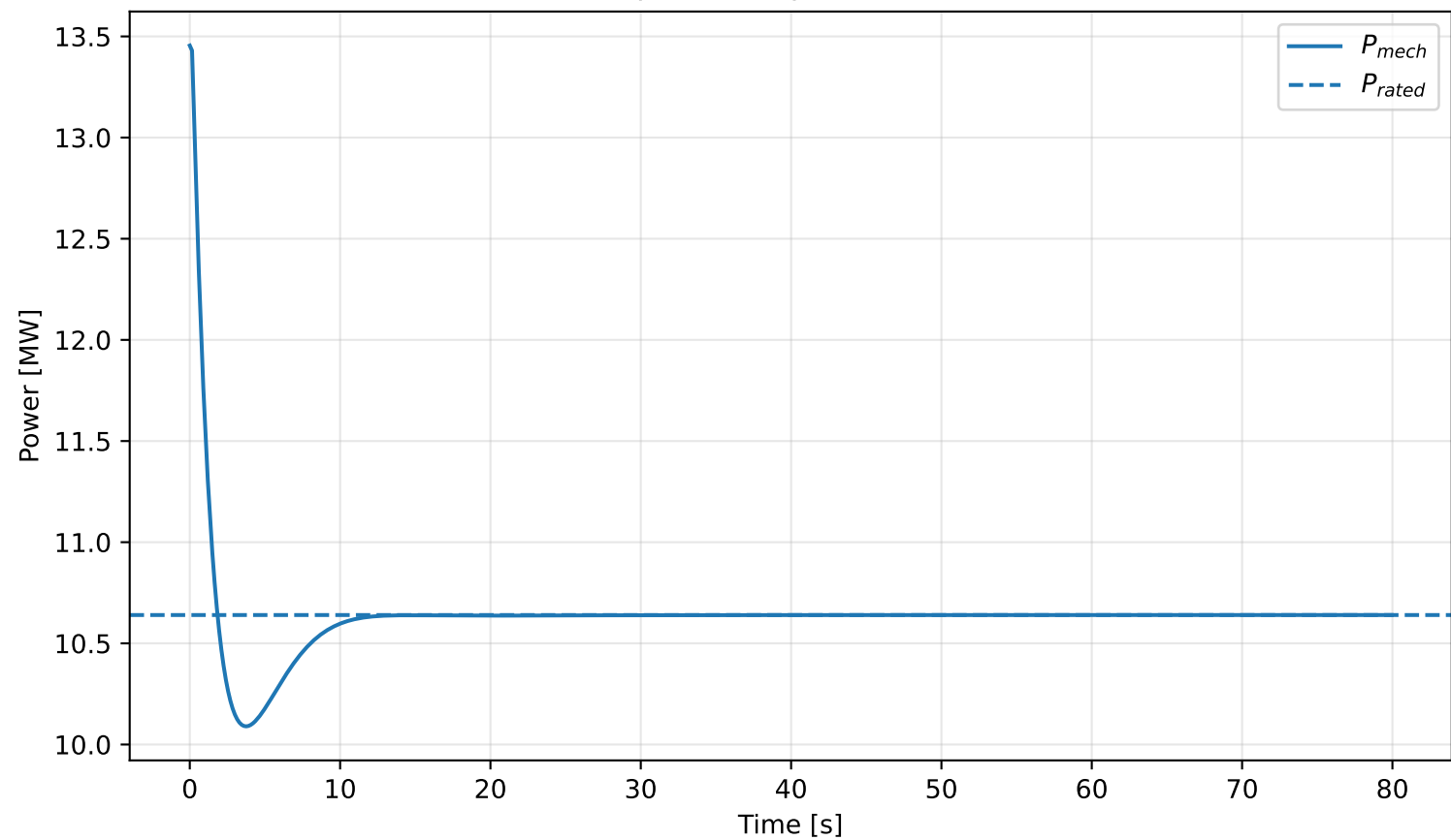
Above-rated power response at V_0 = 16.0 m/s
